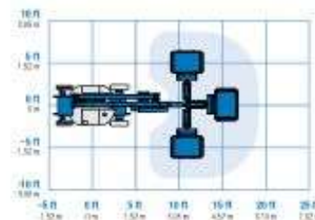
JIB RANGE OF MOTION Z 40/23N RJ
