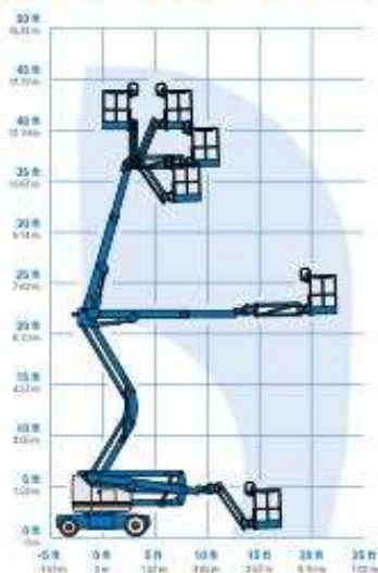
RANGE OF MOTION Z 40/23N RJ
